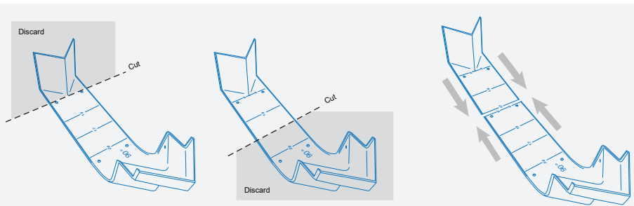
Extend Cast Angles to fit QG150, QG175 and QG200 (Illustration for QG175)
