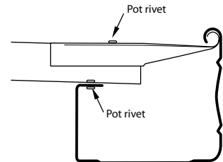
Fascia Guttering with Gutter Bracket
